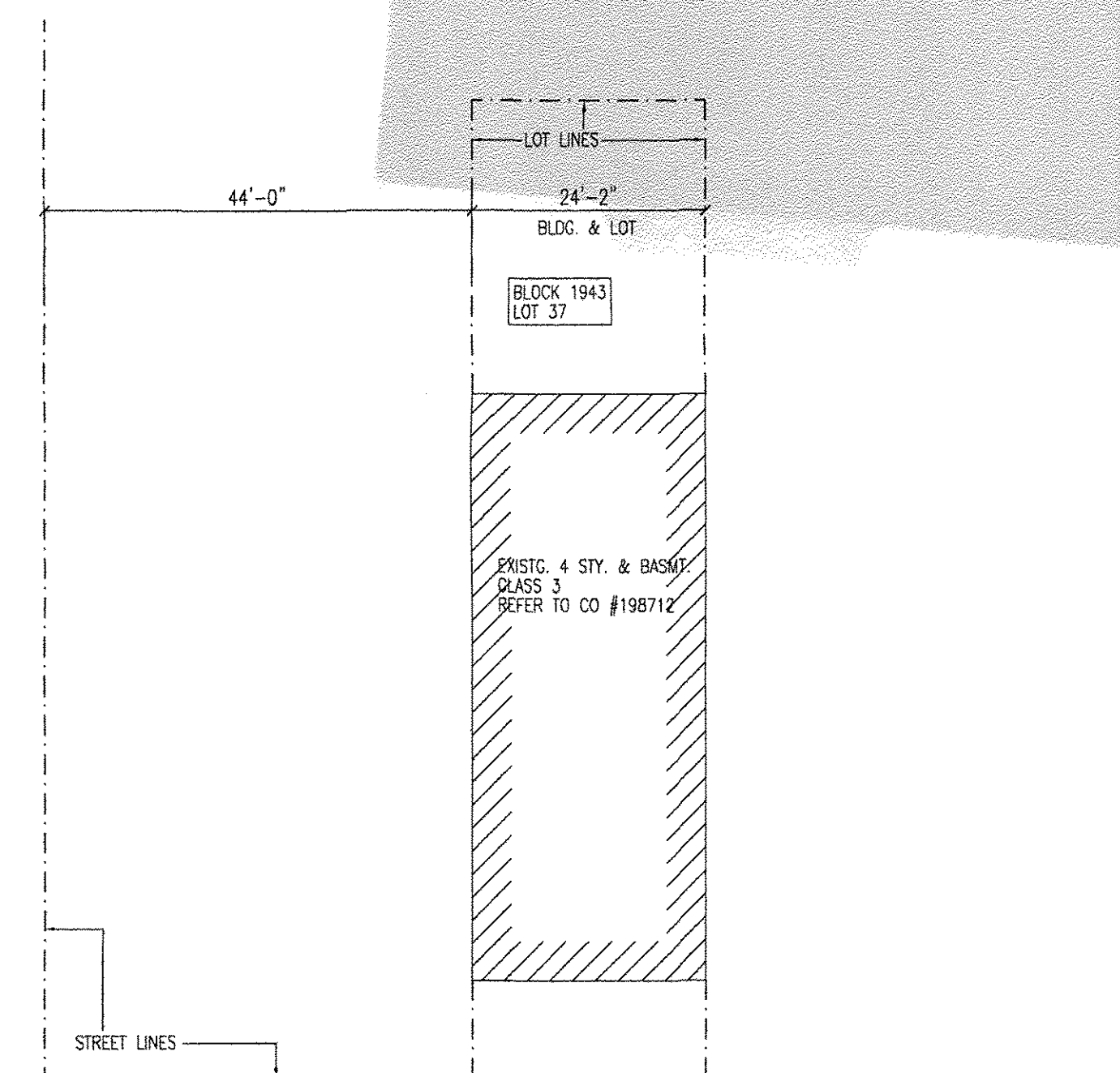
PLOT PLAN SCALE: 1" = 16'-0"
