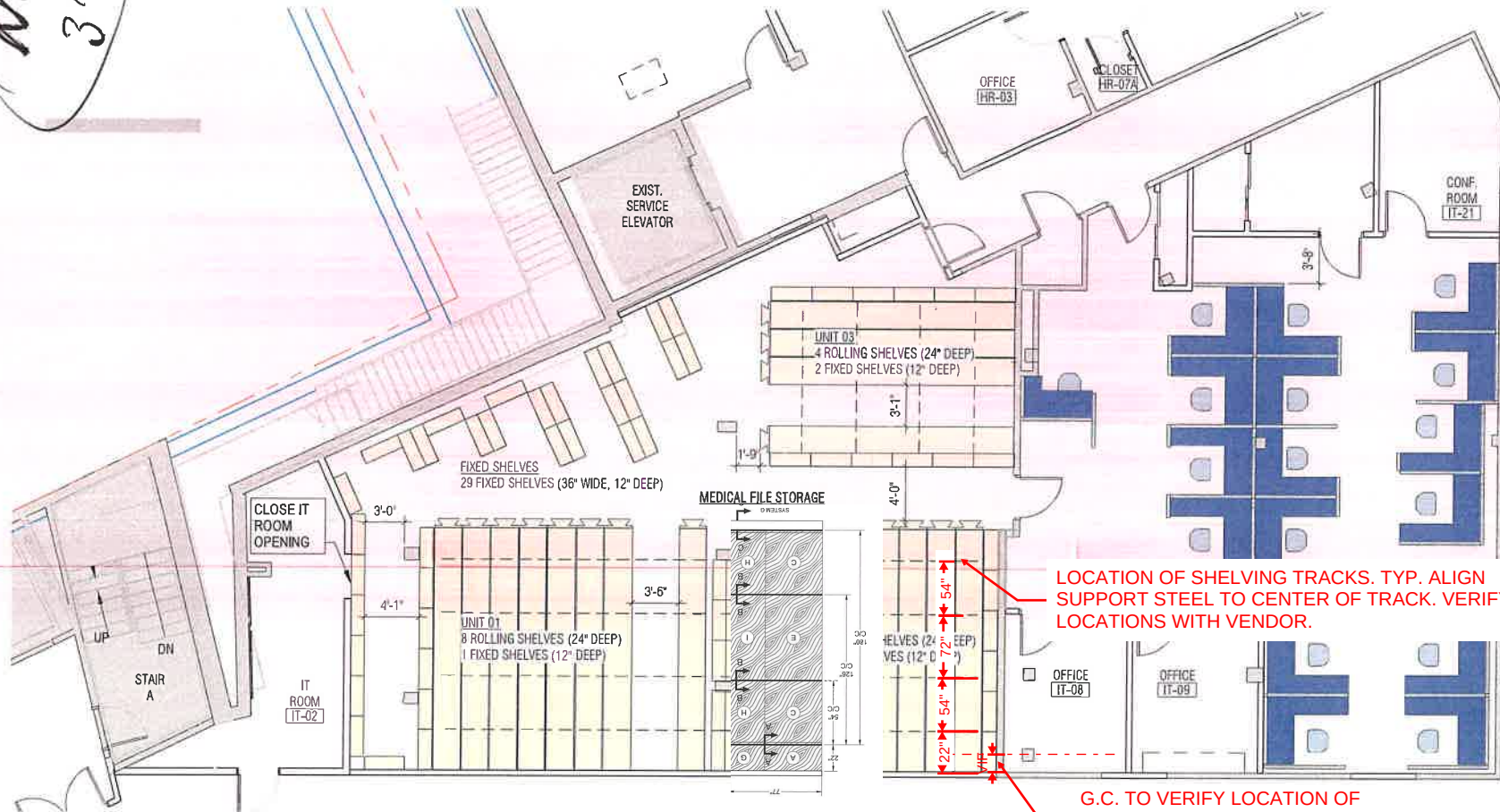
3RD FLOOR CONSTRUCTION PLAN
