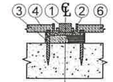
SECTION B-B SCALE 1:8 ROTATED 90° C.W.
