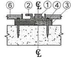
SECTION B-B SCALE 1:8 ROTATED 90° C.W.
