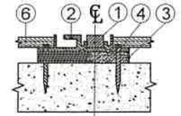
SECTION B-B SCALE 1:8 ROTATED 90° C.W.
