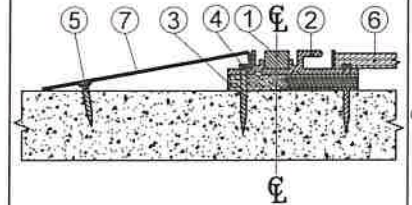
SECTION C-C SCALE 1:8 ROTATED 90° C.W.
