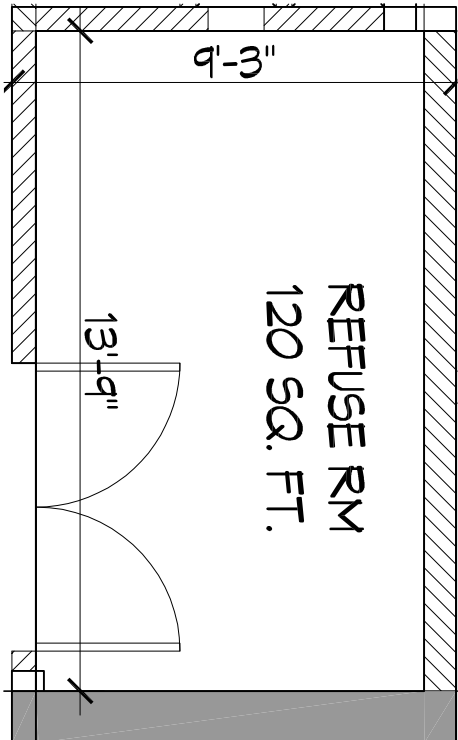
1 REFUSE ROOM PLAN @ CELLAR SCALE - 1/4" = 1'-0"
