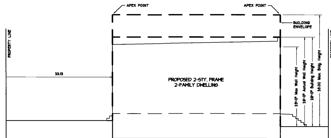
DIAGRAM OF BUILDING ENVELOPE AS PER SECTIONS 23-631 Z.R.
